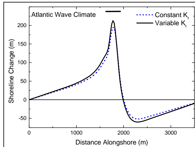
Figure 1. Shoreline change behind emergent detached breakwater (Color figures are allowed)
