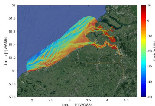
Figure 60: The computational domain and bathymetry of the SCALDIS-COAST model.
