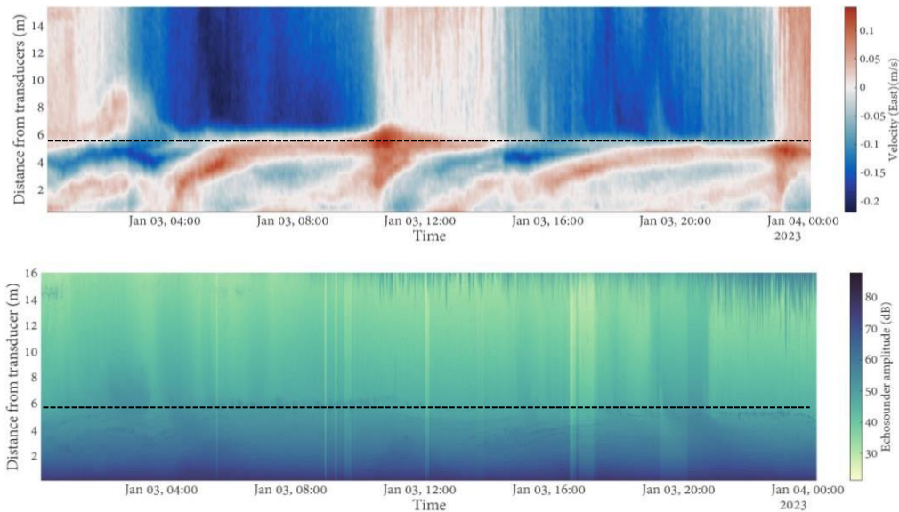
Figure 1: Flow velocity in east-west direction and echosounder amplitudes in a stratified scour hole in the Haringvliet Estuary over one day. The dashed horizontal line indicates the upper part of the scour hole.
