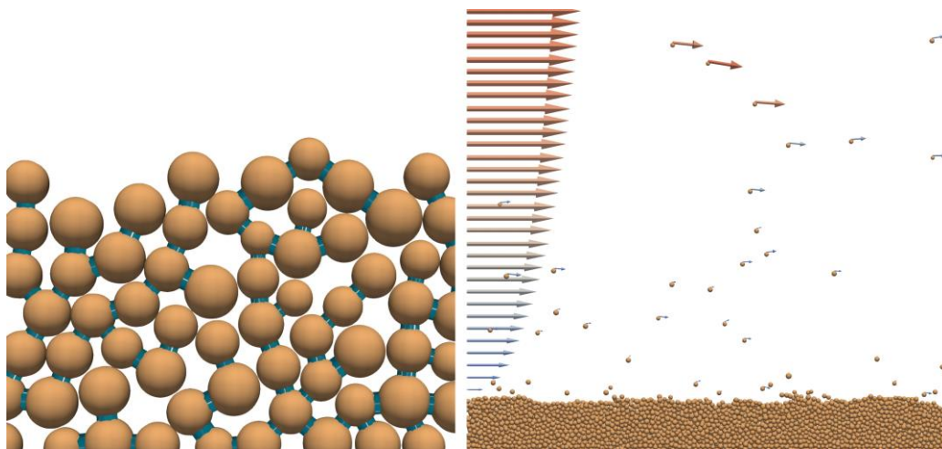
Figure 77: Simulation results in MercuryDPM: left) Sand particles with liquid in between. Right) sand particles being transported by wind (the group of arrows on the left indicates the streamwise wind velocity and the arrows attached to the particles indicate the particle velocities, the larger the size of the arrows, the higher the velocity is).
