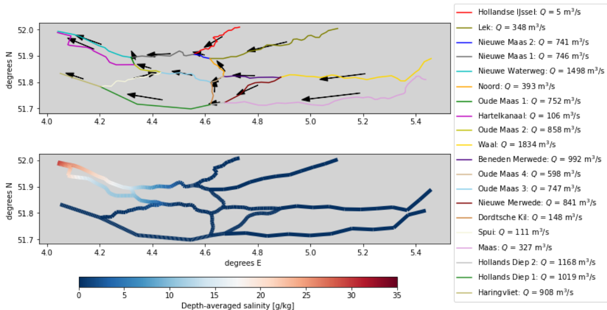
Figure 6: An example of the model results for salt intrusion in the Rhine-Meuse Delta. (a) Discharge in the different branches. (b) Depth and tidally averaged salinity in the different branches.
