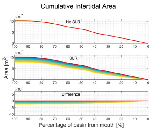
FIGURE 65: CUMULATIVE INTERTIDAL AREA FOR LINEAR SLR = 0.96M/100YEARS. RED LINE INDICATES INITIAL TIME STEP AND YELLOW LINE INDICATES FINAL TIME STEP.
