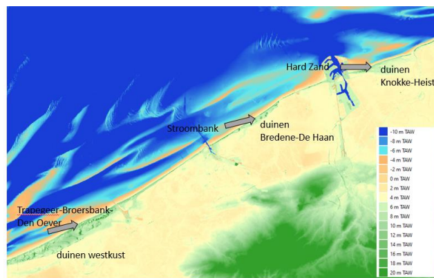
Figure 76: shoreface-connected ridges co-occur with wide dune areas at the Belgian coast
