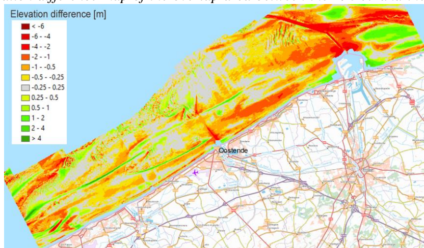
Figure 37: Elevation difference map of the overlap area between the 1984/7 and the 2022 bathymetric
