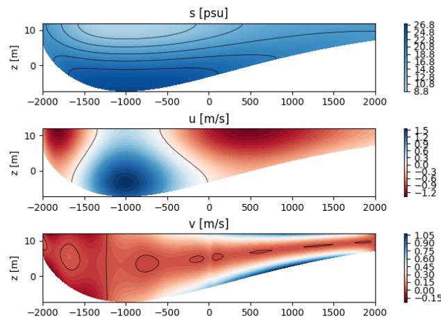
Figure 1: Cross-sectional visualizations of salinity, along-channel flow and cross-channel flow, with salt transport dominated by gravitational circulation inducing lateral circulation through bathymetric variations.
