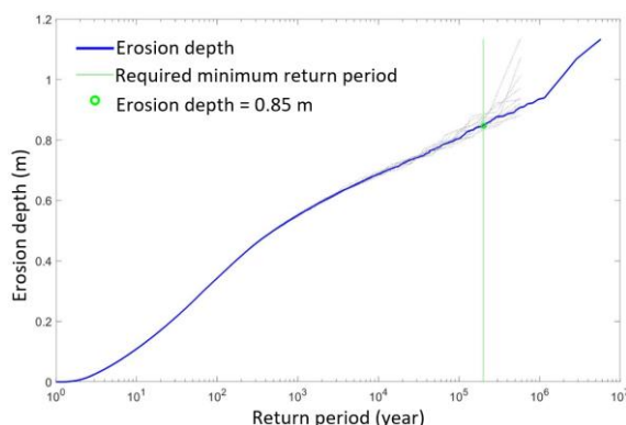
Figure 49: Return period of the erosion depth calculated with the probabilistic model.
