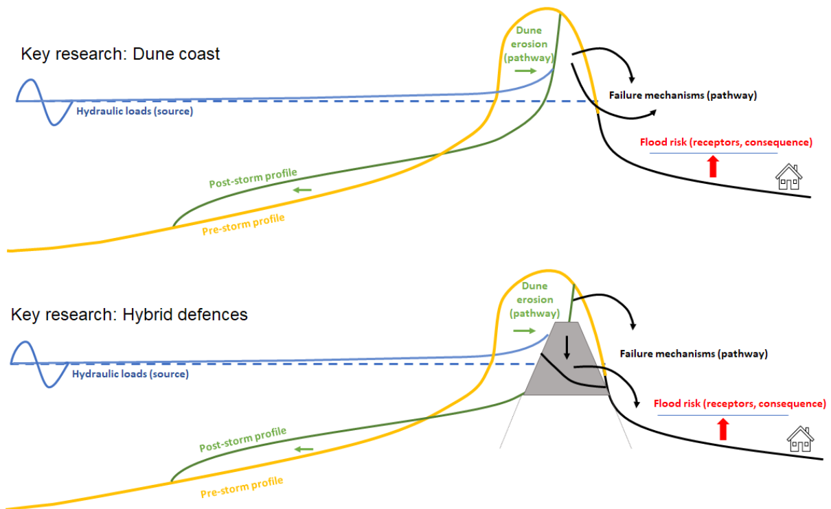
Figure 42: Categorization of research questions in the knowledge agenda in sources (hydraulic loads; blue), pathways (dune erosion, green; further failure mechanisms, black), and receptors and consequences (flood risk, red) for dune coasts and hybrid defences.
