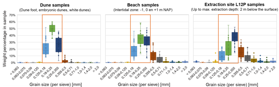
Figure 67: Overview of grain size distribution in the dunes at Vlieland (left), at the beach at Vlieland (middle) and at the sand extraction site for the beach nourishment (right). Orange box indicates the main grain size range in the dunes, which is the potential aeolian transport sand fraction (PATSF).
