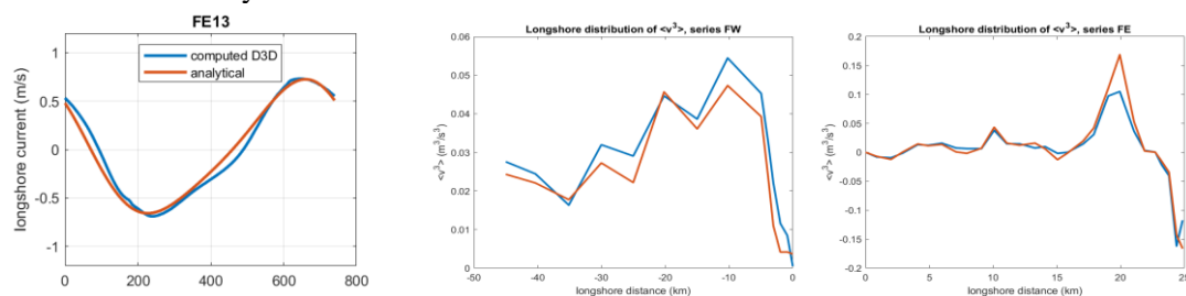
Figure 24: Example time series of tidal velocity (left panel); longshore distribution of tidal velocity skewness, West (middle) and East (right panel) of Zeebrugge
