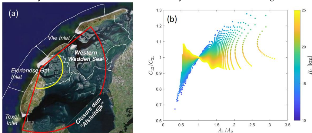
Figure 66: (a) Plan-view of the Western Wadden Sea, including the schematized basin geometry (red) and tidal divide (yellow); (b) Correlation between asymmetry of the inlet connectivities (vertical axis) and asymmetry in inlet areas (horizontal axis) for various basin radii (color).
