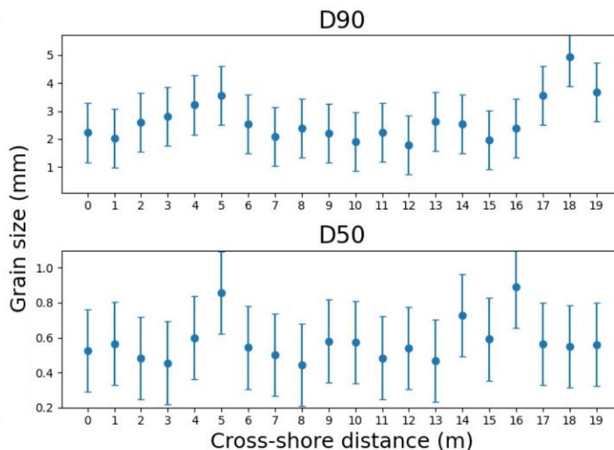
Figure 20: Cross-shore distribution of grain sizes acquired with the new method (note: 0 and 19 m correspond to the high and low waterline, respectively).
