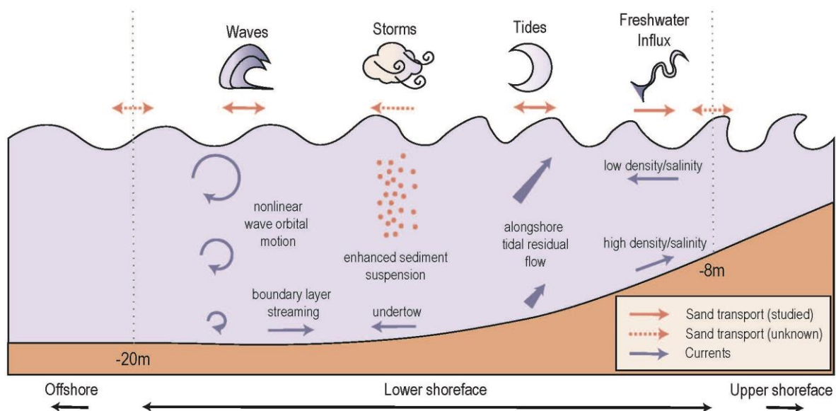
Figure 35: Schematic cross-shore overview of the lower shoreface showing different physical processes with associated net sediment transport direction. In general, these processes are stronger closer onshore.
