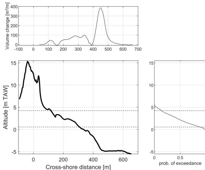
Figure 30: Deposition in relation to the coastal profile during the February 2020 storm. Upper panel: deposited volume in the channel ( m^3/m ). Lower panel: coastal profile (May 2020) and mean high and low water levels (dashed). Right panel: probability of exceedance of the still water level.
