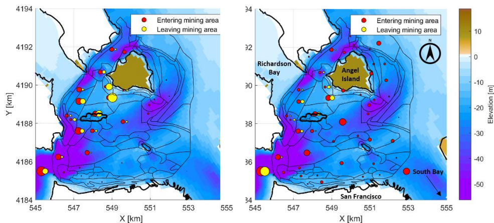
Figure 32: Connectivity of mining ring (black contour below Angel Island) with surrounding areas for (a) 5 tidal cycles and (b) 50 tidal cycles, the size of the dot indicates the strength of the connectivity.
