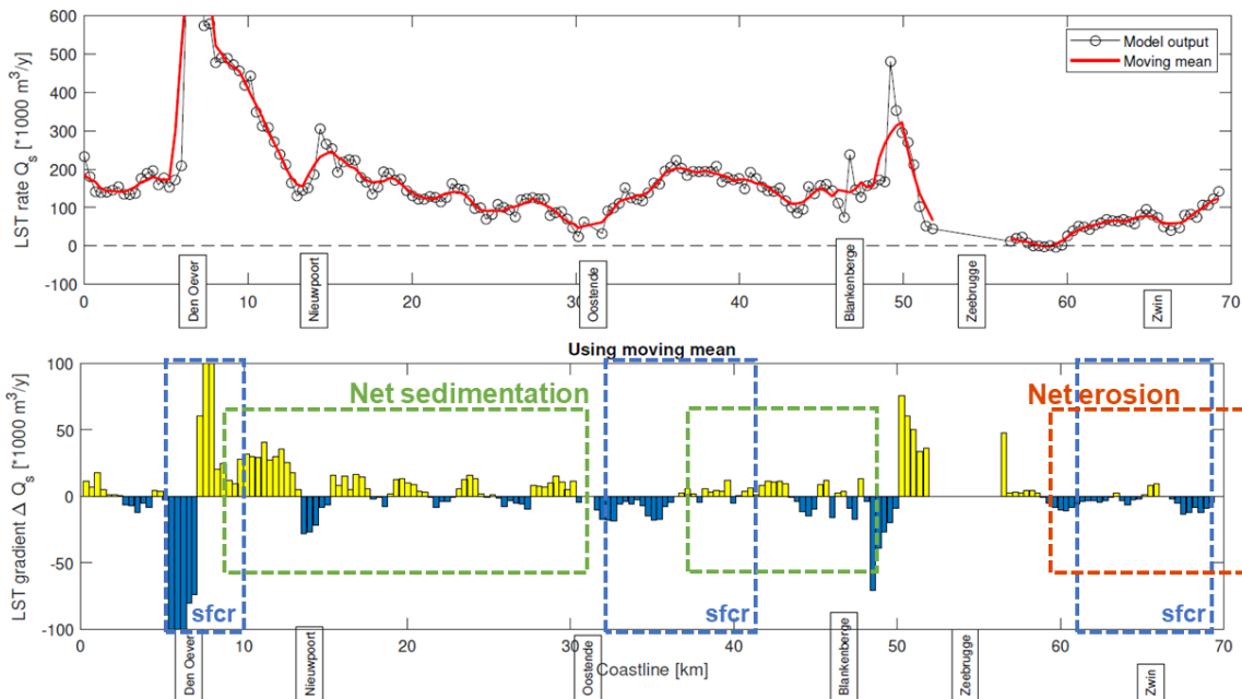
Figure 11: Calculated LST rates (top) and LST gradients (bottom) that can erosion- and deposition locations. The presence of SFCR is shown by blue boxes.
