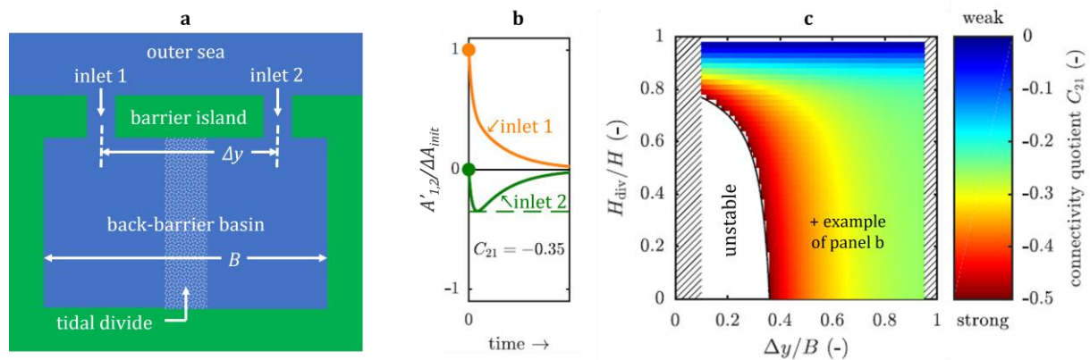
Figure 9: (a) Top view of model geometry showing double inlet system with tidal divide. (b) Example of system's return to equilibrium after perturbing inlet 1, corresponding to a connectivity quotient of C_{21} = -0.35 . The plot shows the time evolution of the perturbations to inlet 1 ( A'_1 in orange) and 2 ( A'_2 in green), scaled with inlet 1's initial perturbation \Delta A_{mit} . (c) Sensitivity of connectivity quotient to inlet spacing \Delta y and tidal divide height H_{div} (scaled with basin width B and depth H , resp.). The example shown in panel b is denoted with +. Red (blue) shades indicate strong (weak) connectivity.
