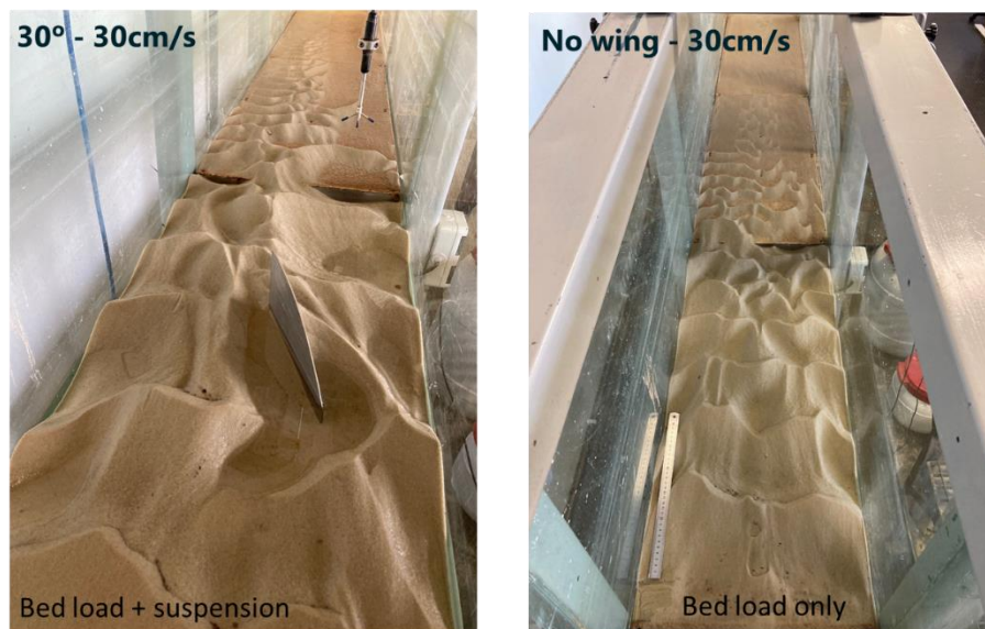
Figure 57: Flume experiments of the Sand Wing with mobile sand bed. Left: Sand Wing with 30° orientation; Right: no Sand Wing. Both experiments were performed with 0.3 m/s flow velocity.
