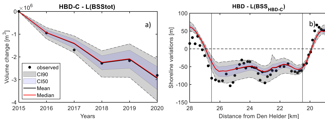
Figure 22: Temporal volume changes over the central sector of the HBD since construction (a), and shoreline position change in the alongshore direction after 5 years (b). Central sector indicated by black vertical lines in panel b.
