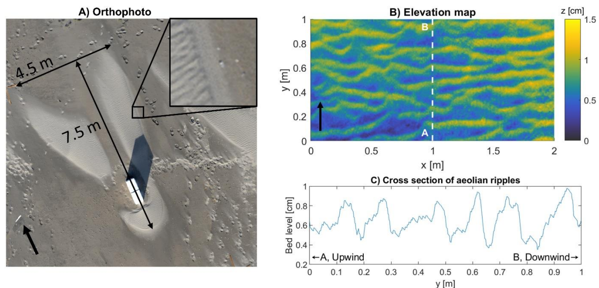
Figure 45: SfM results. A) Orthophoto of deposition (lighter colored sand) around scale models. B) DEM of beach area with aeolian ripples, unaffected by scale models. C) Cross section of the dashed line in B).
