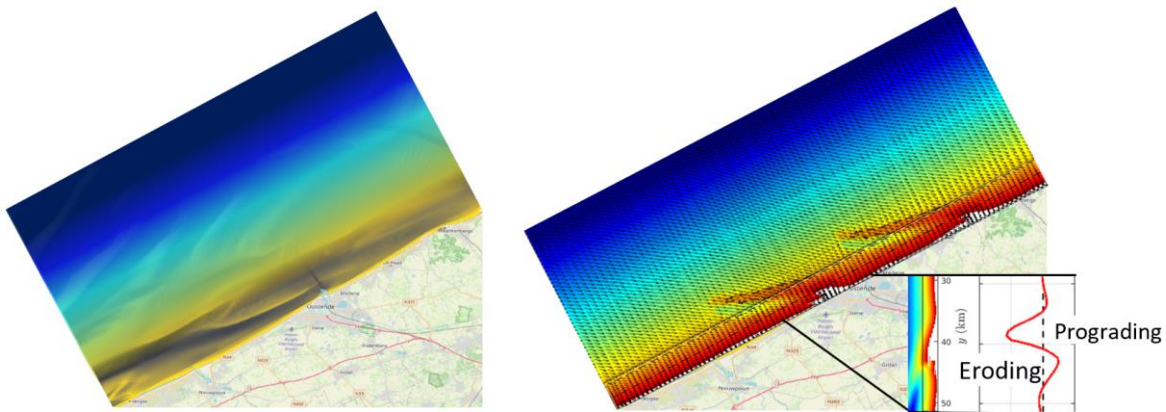
Figure 55: Shoreface-connected sand ridges (SFCR) at the Belgian coast (left) and a typical result of the simulated shoreline evolution in presence of SFCR (right)
