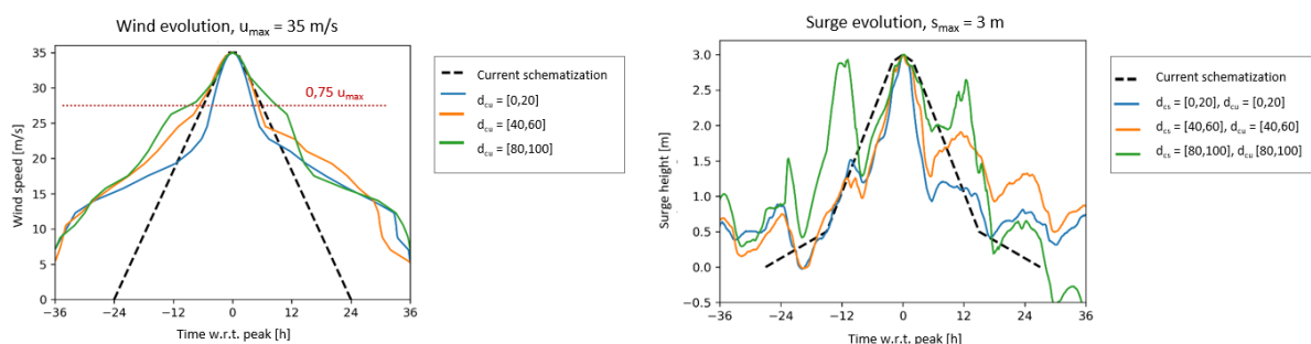
Figure 59: Comparison of the current implementation of the wind and surge evolution in load models for flood defence assessments (dashed lines) and the schematized wind and surge evolutions based on the ECMWF data analyses (coloured lines for different duration classes of wind and surge).
