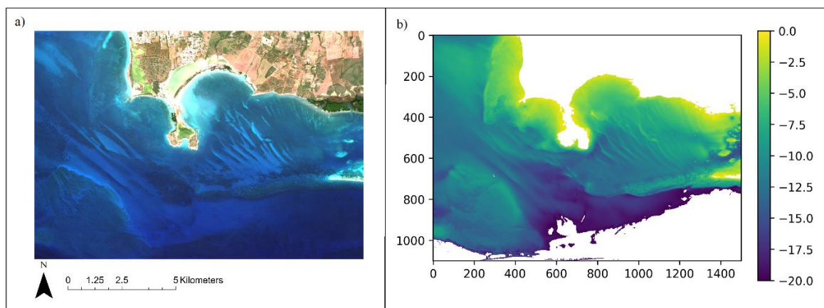
Figure 12: Plots of the median RGB image (a) and predicted depth in meters by XGBoost model (b) of the study area.
