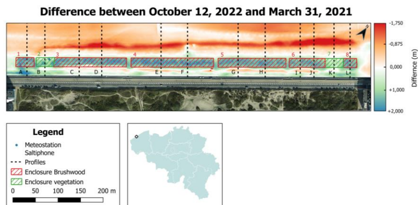
Figure 21: Dune-in-front-of-a-dike pilot site at Raversijde, Belgium divided in 8 zones and 12 cross-shore monitoring profiles.
