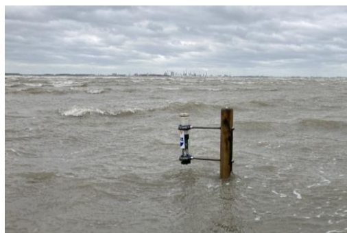
Figure 8: Monitoring short-term sediment dynamics with an acoustic SED-sensor during storm conditions in the Westerschelde (image courtesy: T. Grandjean).
