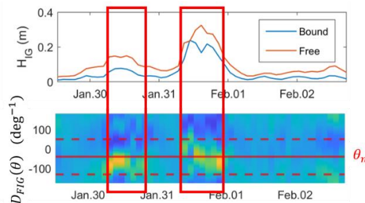
Figure 28: Evolution of bound and free infragravity waveheight (top) and the free infragravity directional distribution (bottom) during storm Corrie (2022). The horizontal line on the bottom panel represents the shorenormal \theta_n , and the dashed lines \theta_n \pm 90 degrees.
