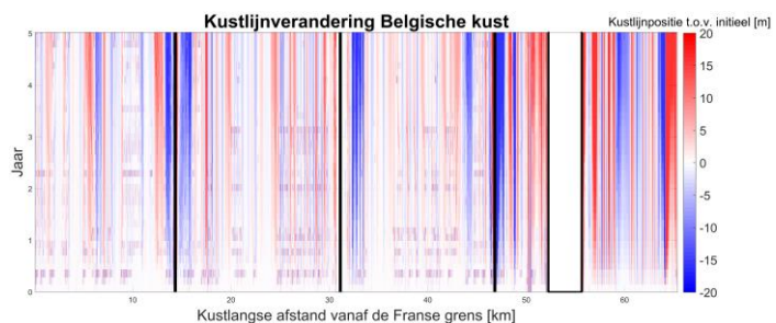
Figure 43: Cumulative evolution of the Belgian coastline, red shows sedimentation and blue erosion.
