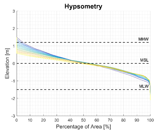
FIGURE 64: HYPOMETRY FOR LINEAR SLR = 0.96M/100 YEARS. BLUE LINE INDICATES INITIAL TIME STEP AND YELLOW LINE INDICATES FINAL TIME STEP.
