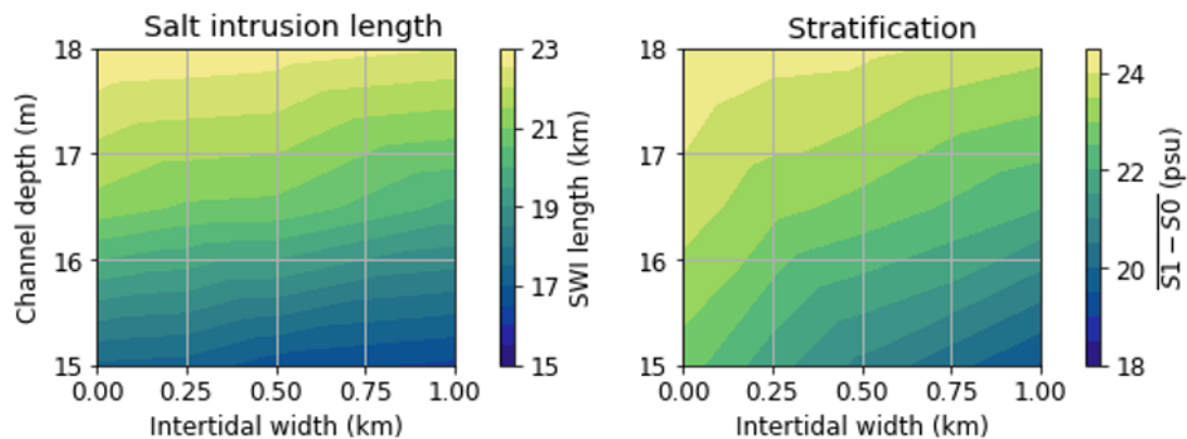
Figure 47: Saltwater intrusion and stratification affected by channel depth and intertidal width
