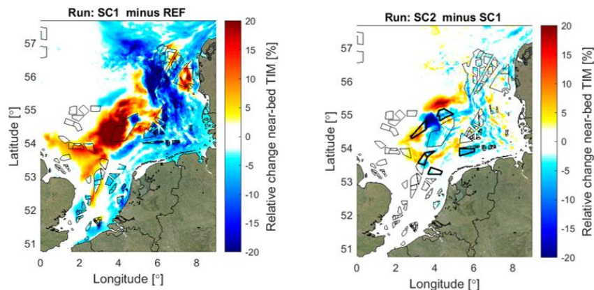
Figure 19: Changes in year-average, near-bed total inorganic matter (TIM) for future wind park scenarios 1 (left) and 2 (right) in 2050.
