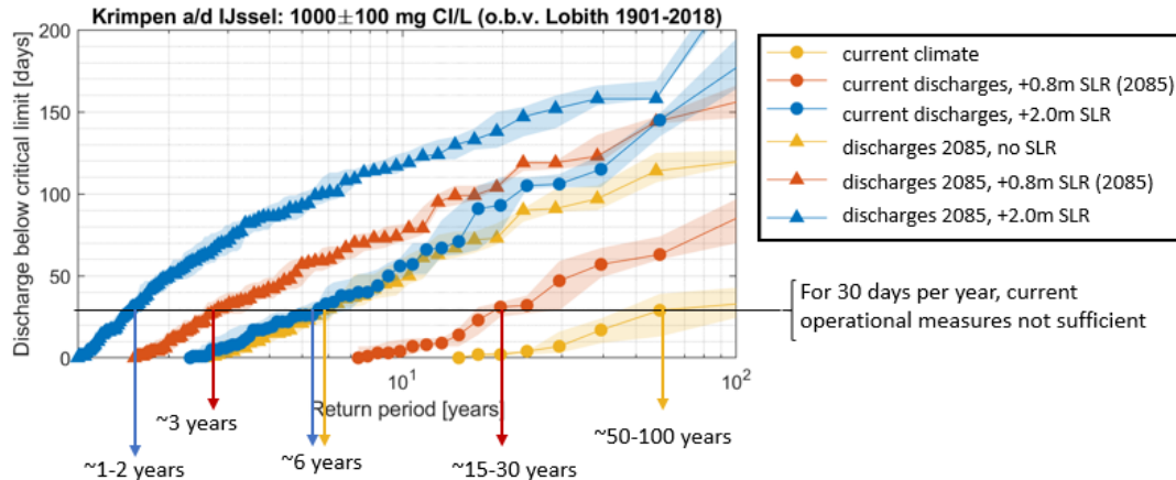
Figure 38: The impact of sea level rise and a changing discharge regime on the return times of salt intrusion events at one of the critical locations for fresh water in the Rhine Meuse Estuary. For sea level rise 0.8 m (high end KNMI'14 projection for 2085) and 2.0 m were taken. The discharge regime projection is based on high-end KNMI'14 projection for 2085 (Sperna Weiland et al., 2015).
