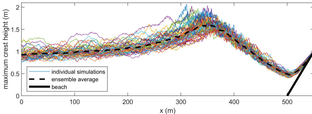
Figure 33: Deterministic variability in maximum wave crest height along a coastal profile.
