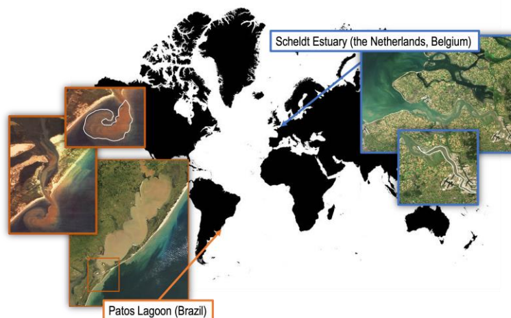
Figure 69: Location of contrasting turbid systems. White contours represent detected coastal features as observed from Landsat (United States Geological Survey – USGS) for Patos Lagoon and Sentinel-2 (European Space Agency – ESA) for the Scheldt Estuary.
