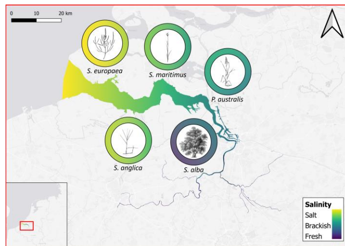
Figure 29: A schematic representation of the Scheldt estuary, showing its salinity distribution and the presence of the five vegetation species at their typical salinity. The illustrations of the vegetation species are not to scale. Salinity data from (Breine et al., 2008). Vegetation illustration courtesy of Lizzie Harper and Botanical-online.
