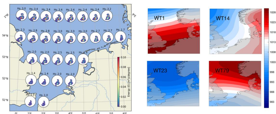
Figure 63: Left: The representative frequency-directional spectra for a specific (grouped) wave condition. The radial axis describes the wave period, with short period waves in the center, the angular axis the wave propagation direction, and the Significant wave heights are based on all the wave energy. Right: The sea level pressure for four characteristic weather conditions.
