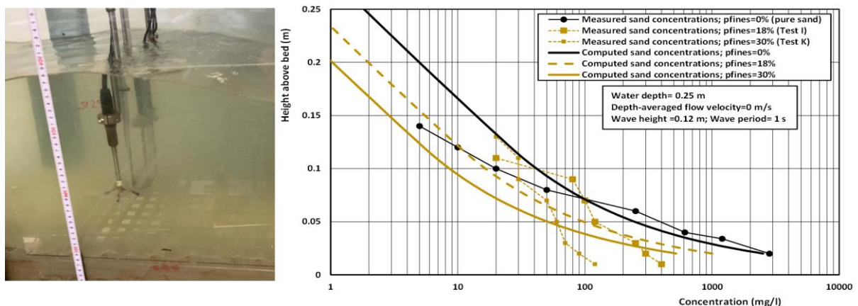
Figure 26: Picture of the experimental set-up in the wave-current flume (left) and comparison between measured and computed sediment concentrations in the flume (right).
