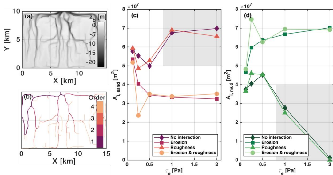
Figure 7: (a) Modelled basin evolution for 1 sand-mud interaction scenario. (b) Extracted reversed Strahler Order of the channel patterns for further analysis. (c-d) Development of the sandy and muddy intertidal areas, depending on the sand-mud interaction settings.
