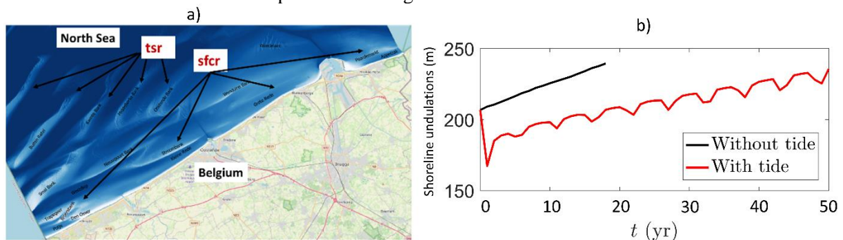
Figure 27: a) Bathymetric map of the Belgian shelf, which shows a field of the so-called shoreface-connected sand ridges (sfcr) and tidal sand ridges (tsr). b) Rms amplitude of shoreline undulations (with respect to the initially straight shoreline profile) versus time.
