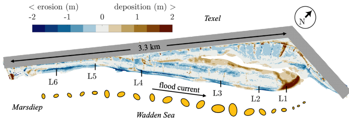
Figure 56: Bed-level change at the Prins Hendrikzanddijk in the first 3 years after construction and a schematic representation of the longshore distribution of cross-shore mean intertidal grain size ( D_{50} = 500\text{-}900 \mu\text{m} ). The black hatched area indicates the location of the old Prins Hendrikdijk.
