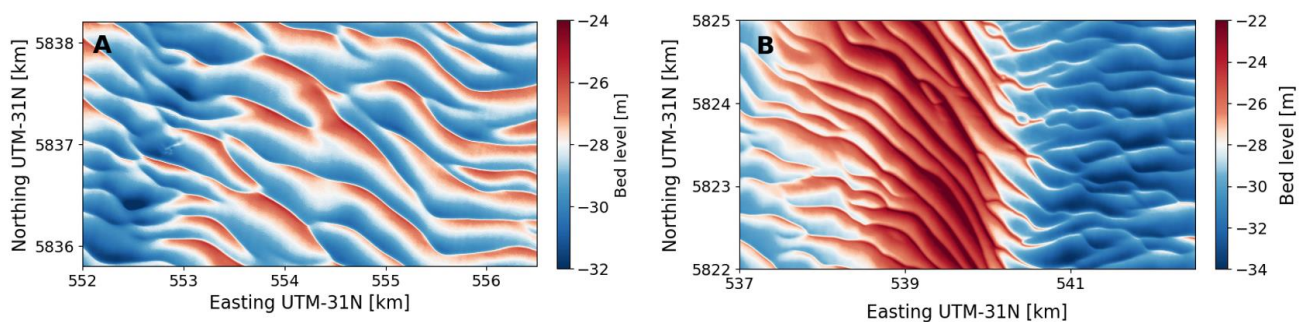
FIGURE 14: MEASURED SAND WAVE BATHYMETRY IN THE NORTH SEA WITH 3D FEATURES (A) AND UNDERLYING SAND BANK (B)
