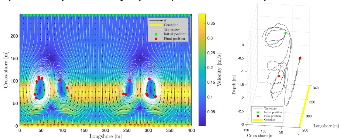
Figure 23: Left: Lagrangian flow field in the nearshore zone of Duck and the resulting trajectories of floating particles released at the offshore boundary without the effect of turbulence. Right: Trajectories of 3 sinking particles released close to a rip cell with added turbulence.
