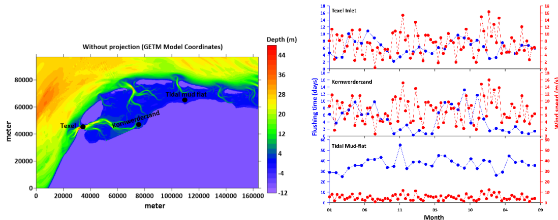
Fig 1. Bathymetry and local flushing time at three different regions of the Dutch Wadden Sea
