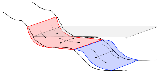
Figure 25: Conceptual model of sediment transport at low-energy, non-tidal, sandy beaches during storm
