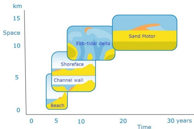
Figure 58: Spatial and temporal scales on which the various types of nourishments act.
