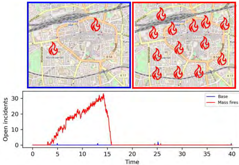
Figure 2: Visualization of the results of the simulation of authority processes. Inspected is an exemplary fire brigade which is sufficiently equipped to extinguish fires under normal circumstances (top left), allowing for immediate response to all fires (bottom, blue curve). Once heavy sabotage during a hybrid crisis causes a lot of fires at the same time (top right), the fire brigade gets overwhelmed, and several fires stay untreated for some time (bottom, red curve).
